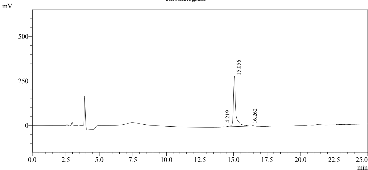
Chromatogram
