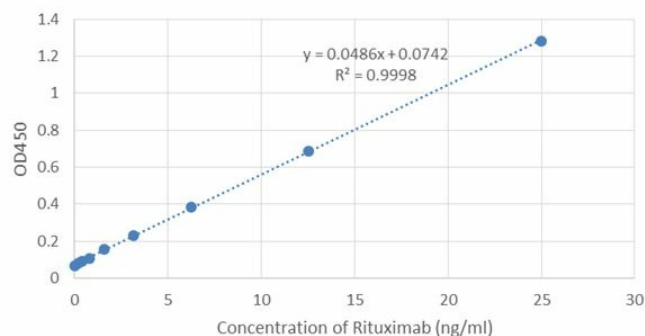
Standard curve of Rituximab Sandwich ELISA
