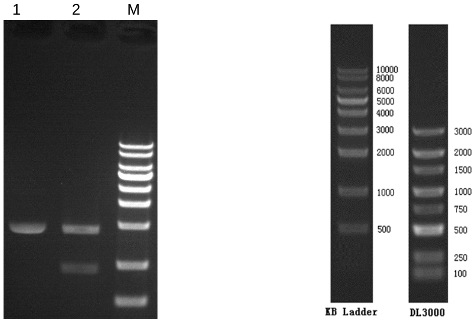
Lane M: KB Ladder Lane 1: U122AGK010-1 plasmid Lane 2: U122AGK010-1 plasmid digested by EcoRI and ScaI
