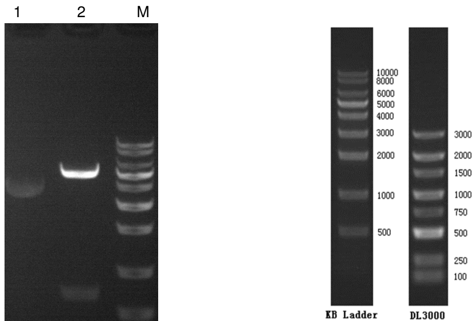
Lane M: KB Ladder Lane 1:U0252GD080-1 plasmid Lane 2:U0252GD080-1 plasmid digested by MluI and HindIII
